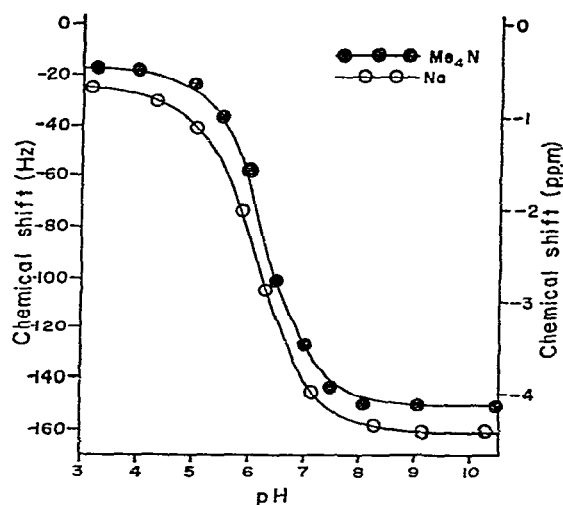
Fig. 3. ^{31}\text{P} n.m.r. titration curves of the monoester groups in partially hydrolyzed O -phosphonomannan YB-2097. [The curves show the effects of the sodium and tetramethylammonium counter-cations on the acid strength of the weakly acidic phosphate functional-groups.]
