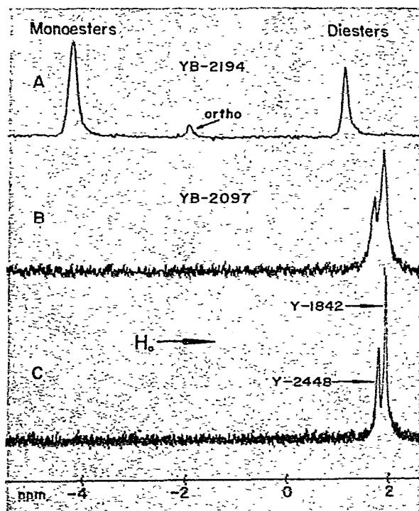
Fig. 1. ^{31}\text{P} n.m.r. ^1\text{H} , broad-band, decoupled spectra of O -phosphonomannans in 0.1M EDTA ( \text{Na}^+ counter-cation) at neutral pH. [A, partially degraded O -phosphonomannan YB-2194; B, O -phosphonomannan YB-2097 containing 2 different types of side chain; C, a 1:2 (v/v) mixture of 2 different O -phosphonomannans, Y-2448 and Y-1842. The samples were \sim 0.02\text{M} in phosphorus ( \sim 400 mg of O -phosphonomannan per ml), and Fourier-transform spectroscopy was used to obtain the spectra: sweep-width, 500 Hz (dwell time 1,000 \mu\text{sec} per point, for 8,192 data points); cycling time, 9 sec; total signal-averaging time, 2–3 h. ^2\text{D} field-frequency stabilization was employed, using the HOD signal from the solvent (10% of \text{D}_2\text{O} added to the sample). Zero p.p.m. corresponds to the resonance position of external, 85% orthophosphoric acid.]
