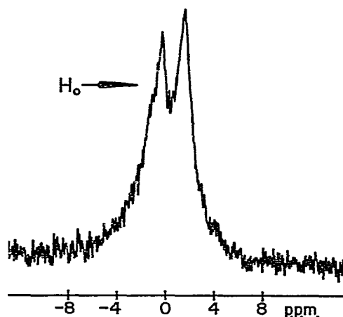
Fig. 2. ^{31}\text{P} n.m.r. ^1\text{H} , broad-band, decoupled spectrum of washed cells of H. holstii NRRL Y-2155. [The sample tube contained packed cells in a medium of 0.05M potassium chloride (pH 7). Fourier-transform, spectroscopic techniques were used with field-frequency stabilization provided by the deuterium signal from acetone- d_6 in a sealed capillary tube coaxially mounted in the sample cell: sweep-width, 2.5 kHz (200 \mu\text{sec} per point, 4,096 data points per spectrum); cycling time, 823 msec; signal averaging time, \sim 2 h. Chemical shifts are in reference to 85% orthophosphoric acid.]
